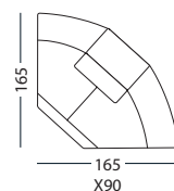
BW1L-1,5RPO-1,5NO-X90K-1,5NO-1,5RPO-BW1P
